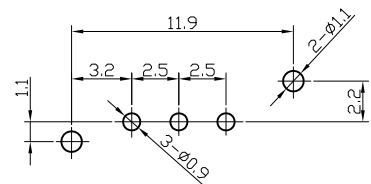
HOLE LAYOUT TOP VIEW
