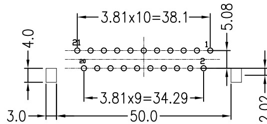
PCB HOLE PATTERN
