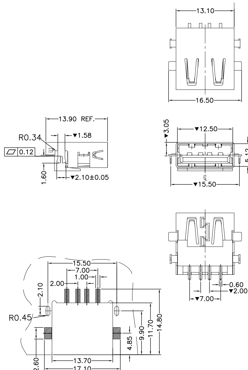
Recommended P.C.B Pattern Layout
